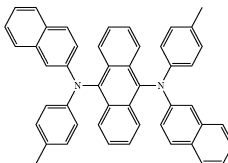
[chemical formula 3]
